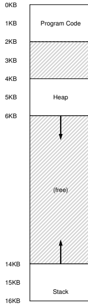
Figure 15.1: An Address Space (Again)
