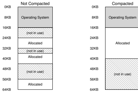
Figure 15.3: Non-compacted and Compacted Memory.
