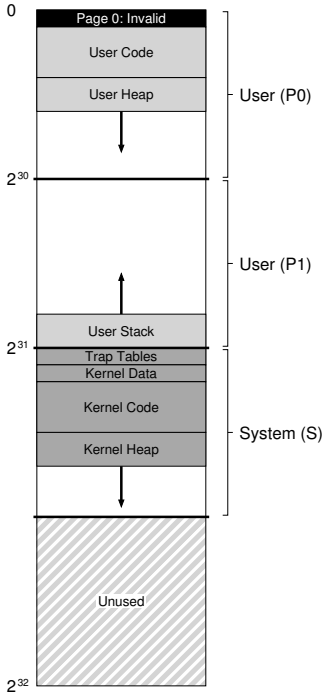
Figure 22.1: The VAX/VMS Address Space
