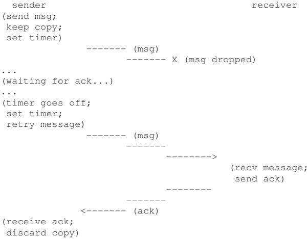
Figure 46.4: Message Plus Acknowledgment
