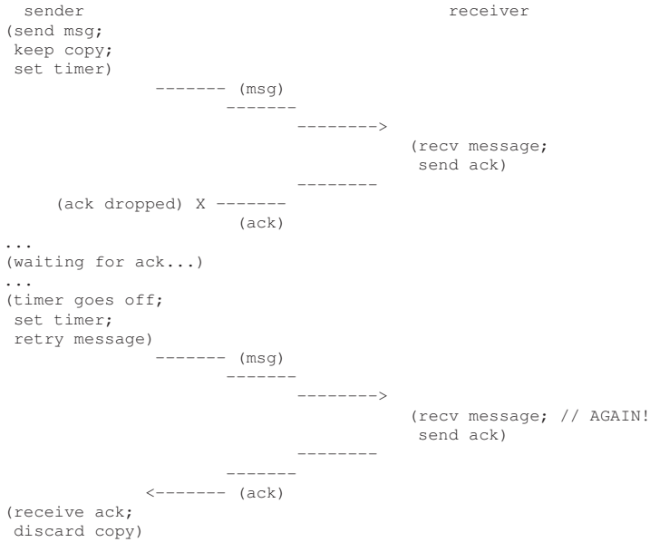
Figure 46.5: Message Plus Acknowledgment
