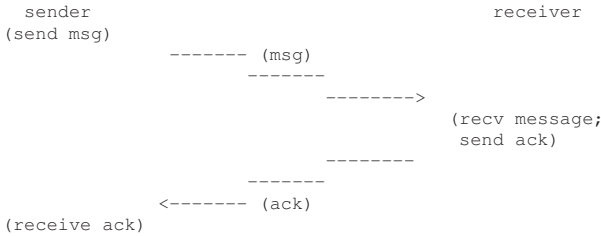
Figure 46.3: Message Plus Acknowledgment
