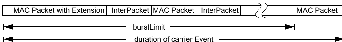
Figure 4–4—Packet bursting
