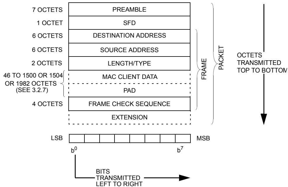
Figure 3–1—Packet format
