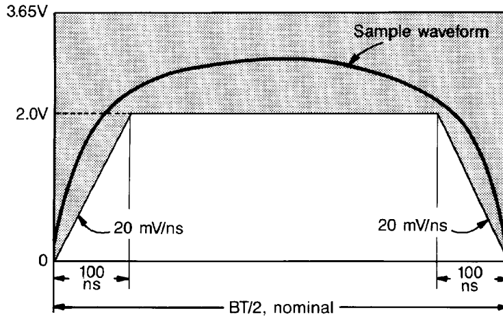
Figure 12-19—Differential output voltage, nominal duration BT/2
