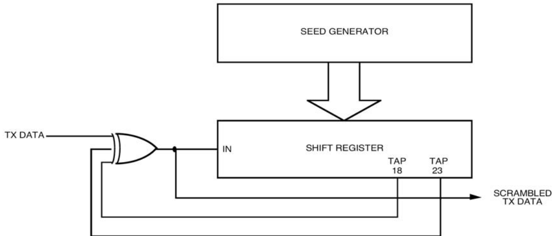
Figure 11–10—Scrambler
