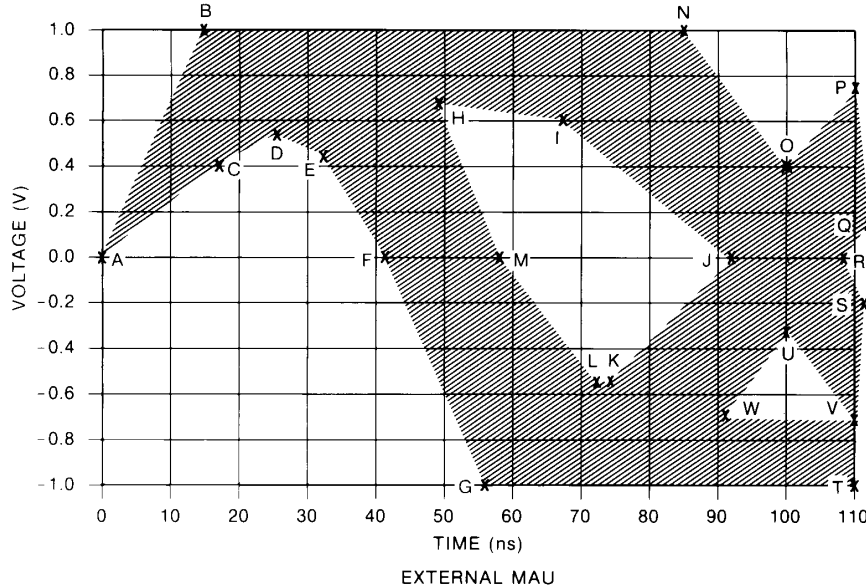
Figure 14–9—Voltage template
