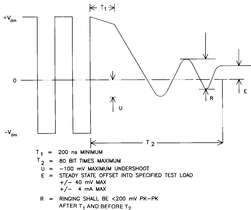
Figure 7-12—Generalized driver waveform
