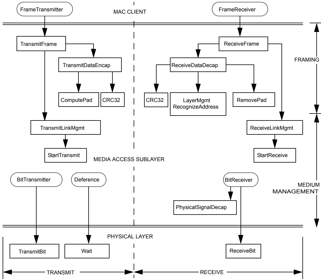
Figure 4A-1—Relationship among MAC procedures
