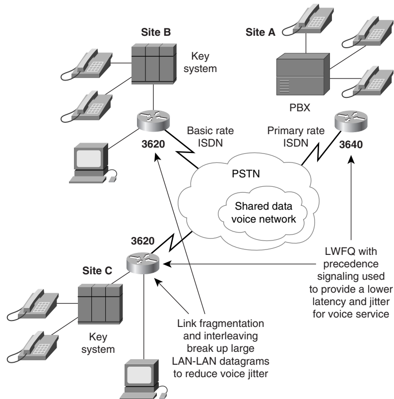
Figure 49-17 This Diagram Provides an Overview of a QoS VoIP Solution
