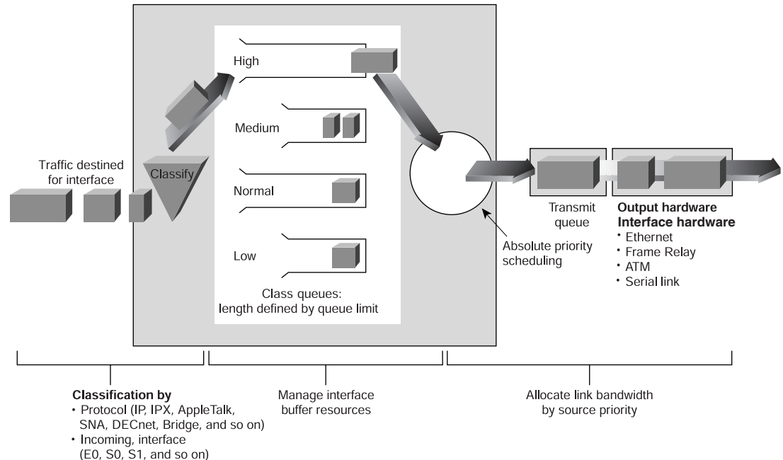
Figure 49-6 Priority Queuing Places Data into Four Levels of Queues: High, Medium, Normal, and Low
