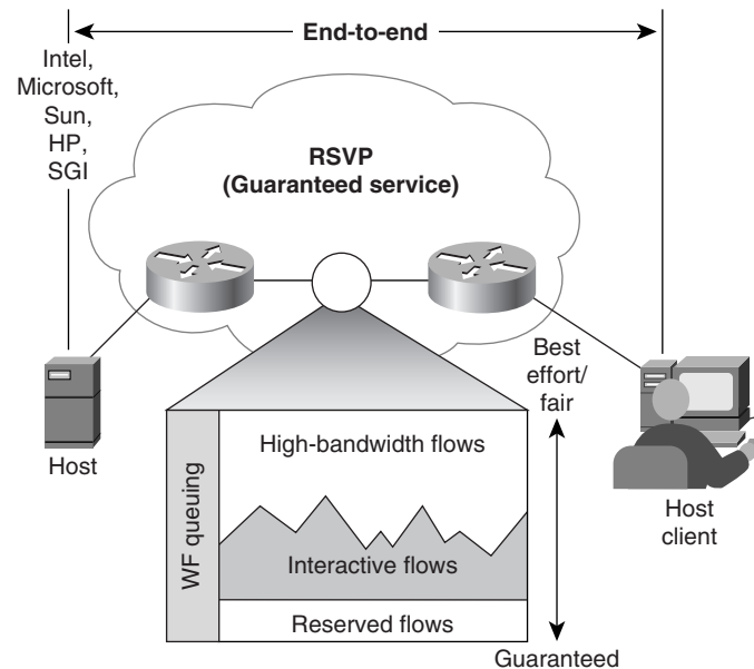
Figure 49-14 This Figure Shows RSVP Implemented in a Cisco-Based Router Network
