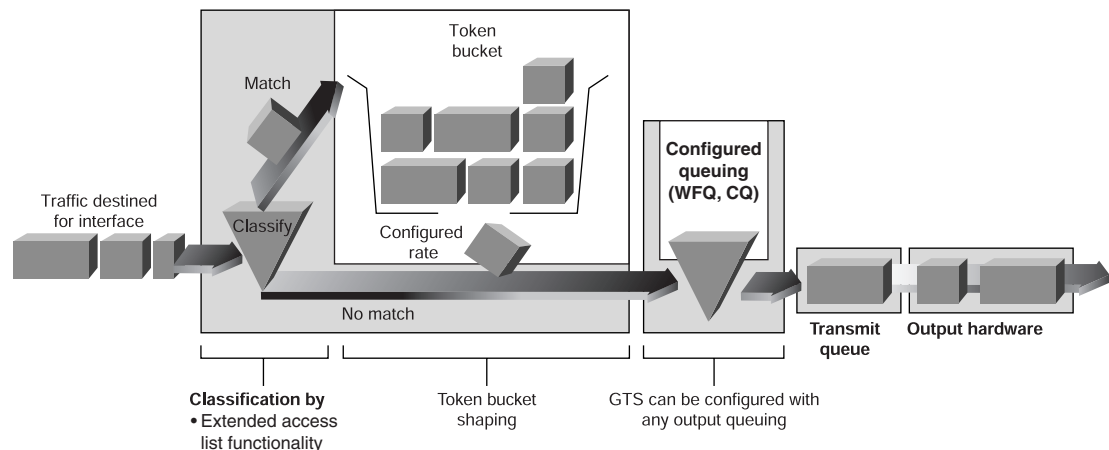
Figure 49-11 Generic Traffic Shaping Is Applied on a Per-Interface Basis
