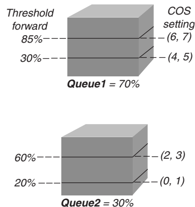
Figure 49-15 WRR with WRED Using Two Queues with Two Thresholds Each
