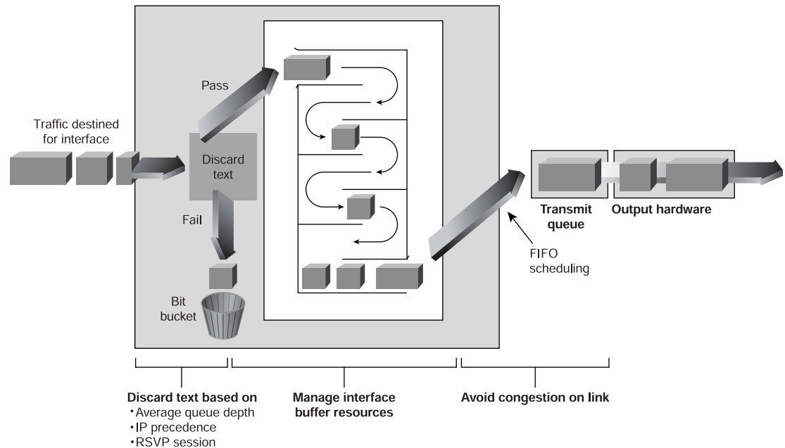
Figure 49-10 WRED Provides a Method That Stochastically Discards Packets if the Congestion Begins to Increase
