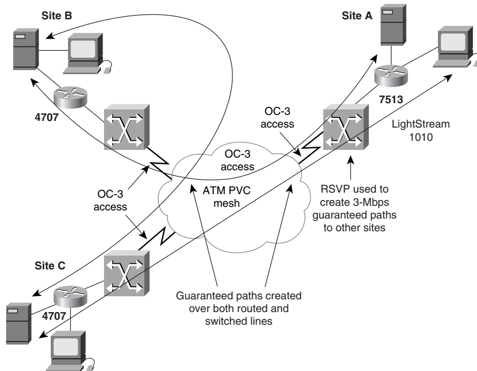
Figure 49-18 The Network Diagram Shows the Use of RSVP in a Meshed ATM Environment
