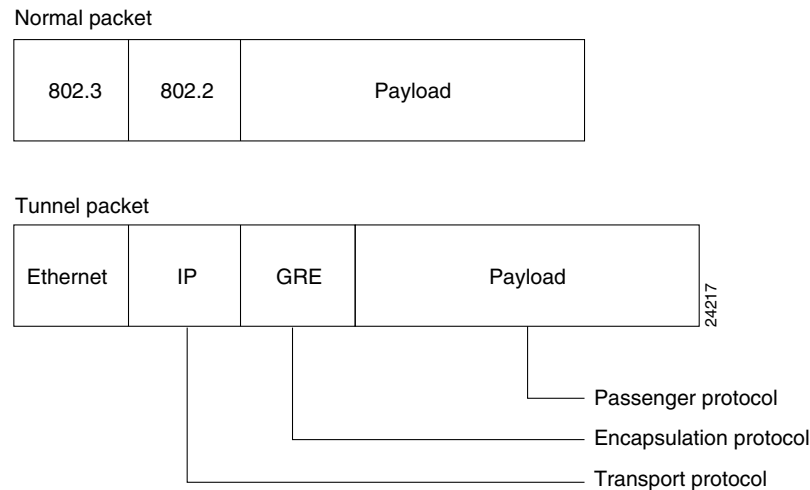
Figure 3-5 IP Tunneling Terminology and Concepts
